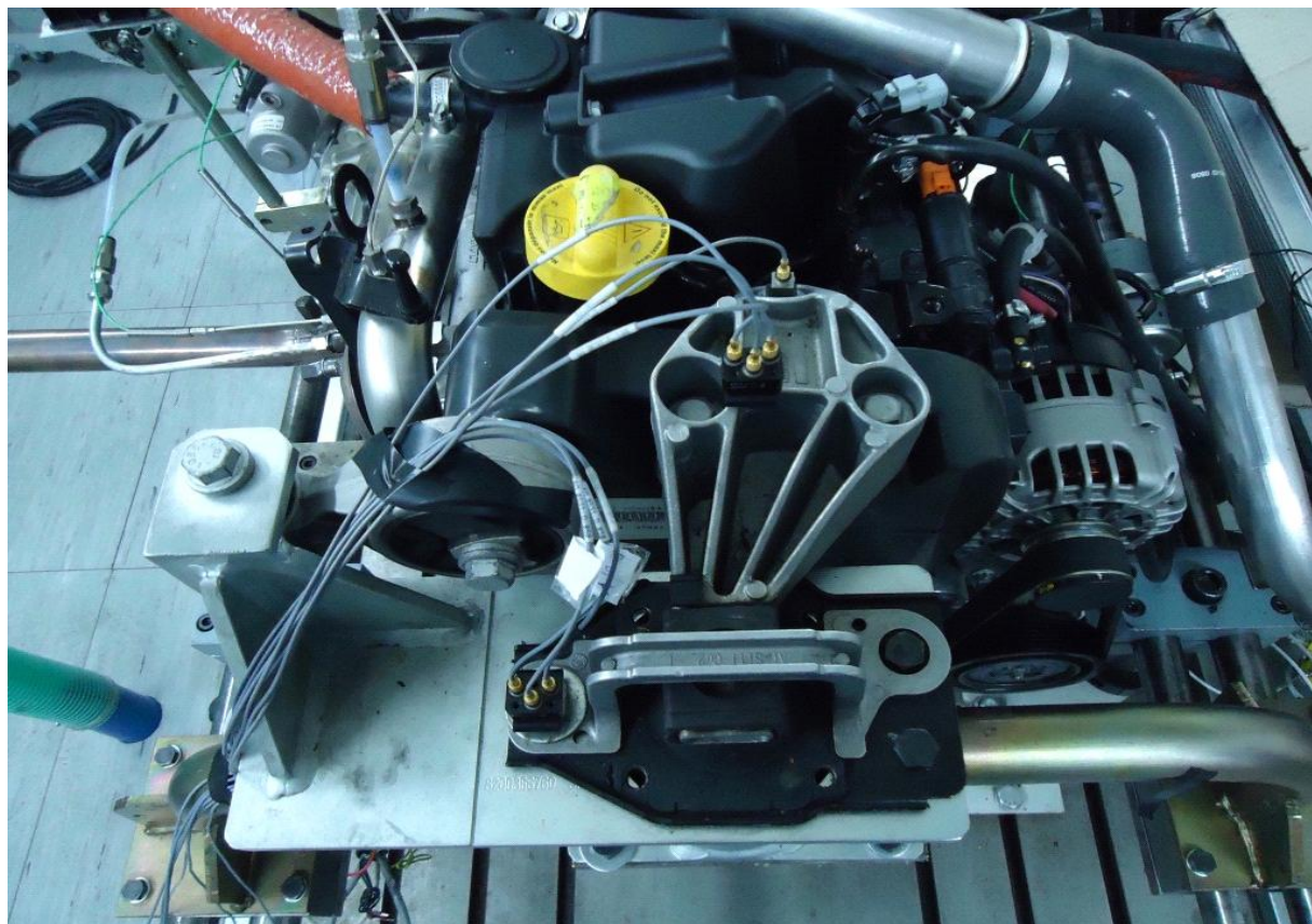
Figure 3. Sensors positioning
